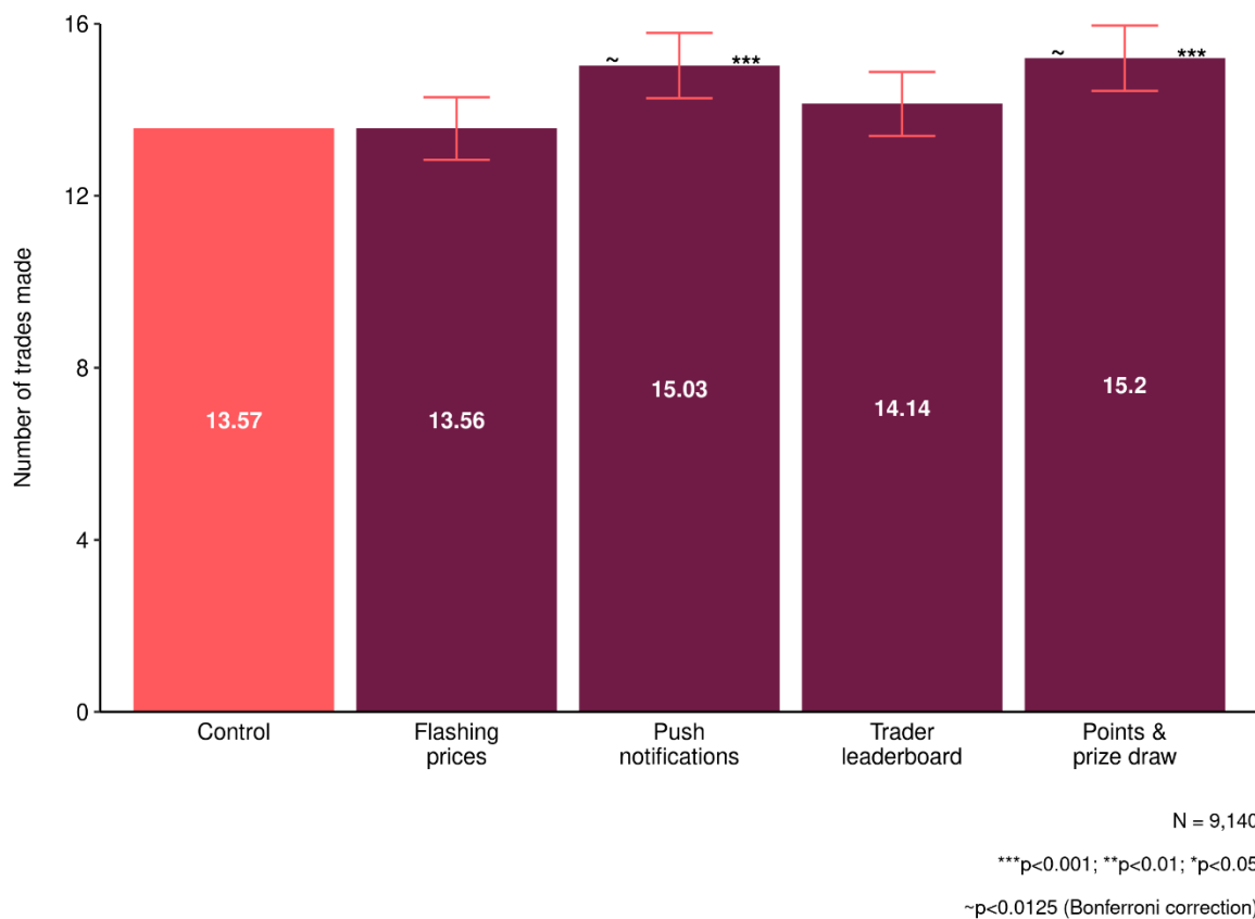
Figure 10. Trading Frequency
