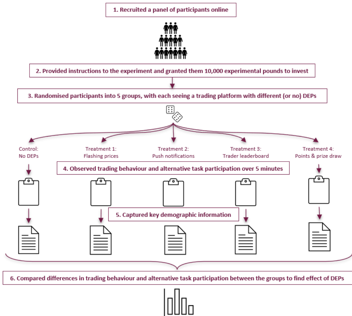
Figure 1: Experiment flow
